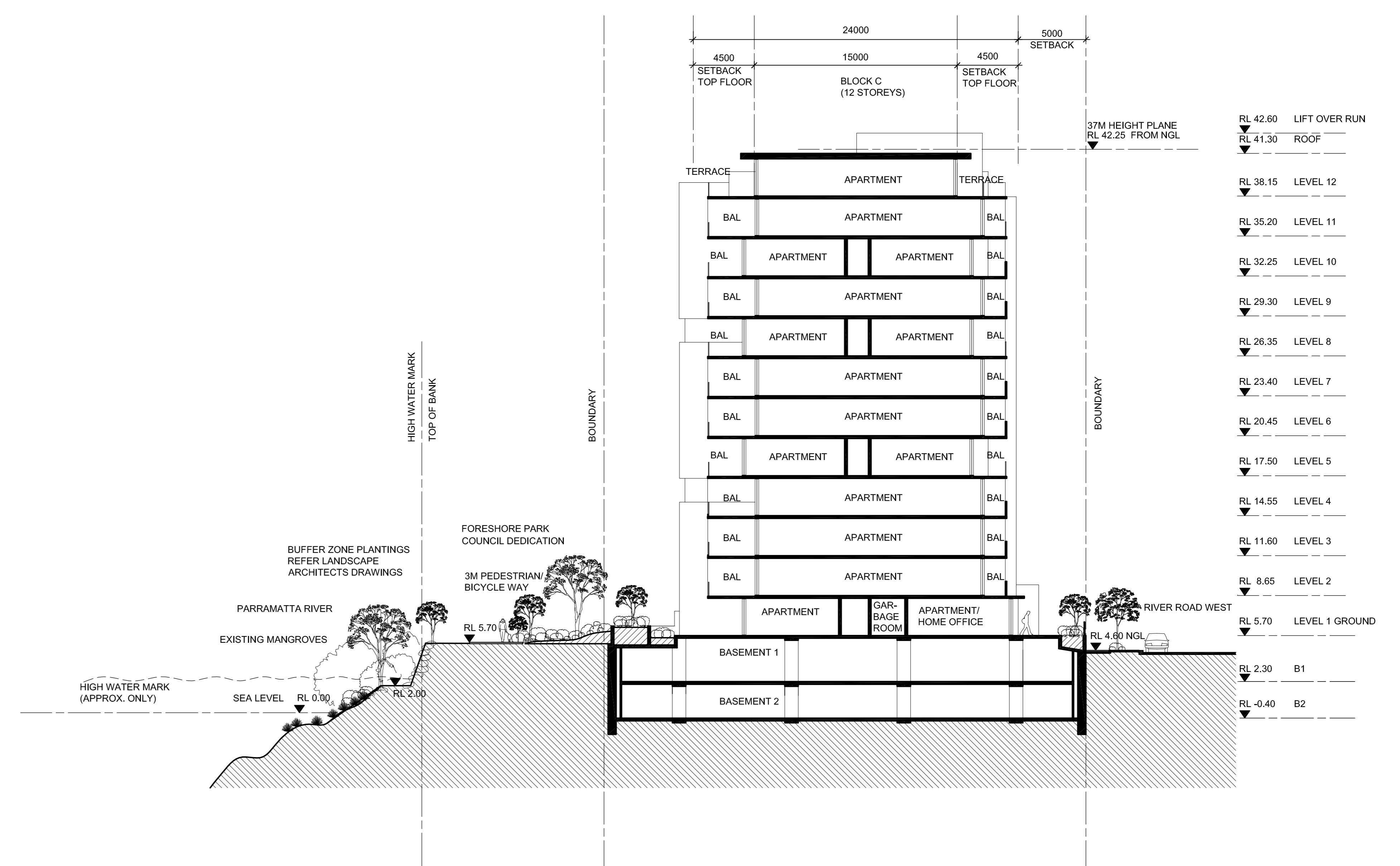
02 SECTION B-B
