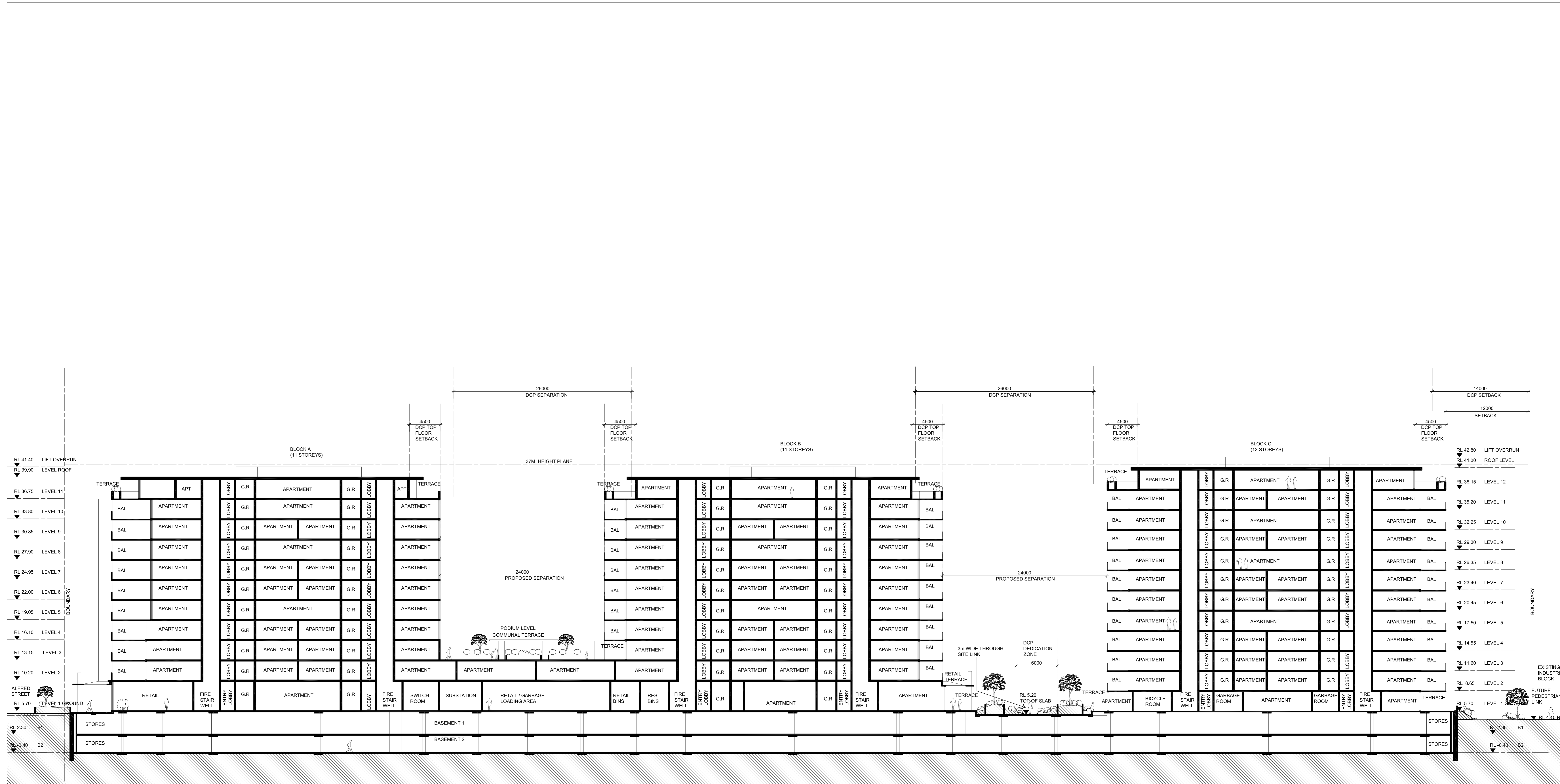
01 SECTION C-C
